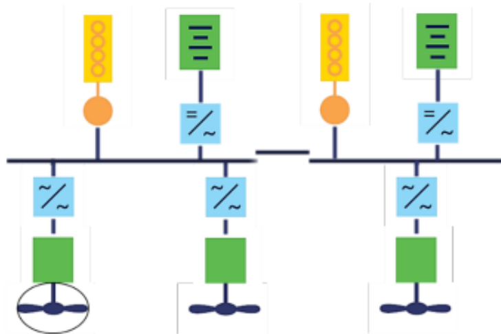
Figure 77: Battery hybrid propulsion
