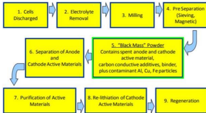
Figure 99 Direct recycling technology from Farasis energy 453
