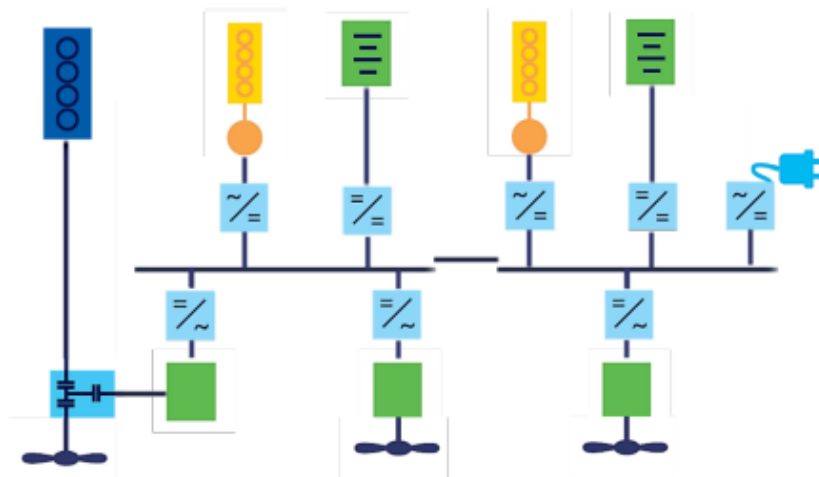
Figure 79: Electrical/mechanical hybrid with DC power distribution
