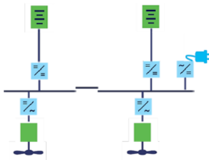
Figure 80: All-electric propulsion
