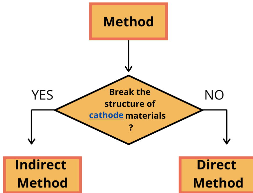
Figure 97 Direct and indirect method to recycle Li-ion batteries
