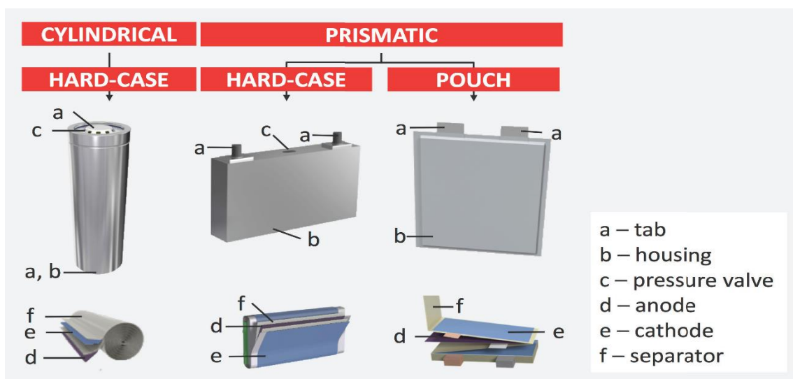
Figure 47 Different cell geometries for LIBs. According to the source. 263
