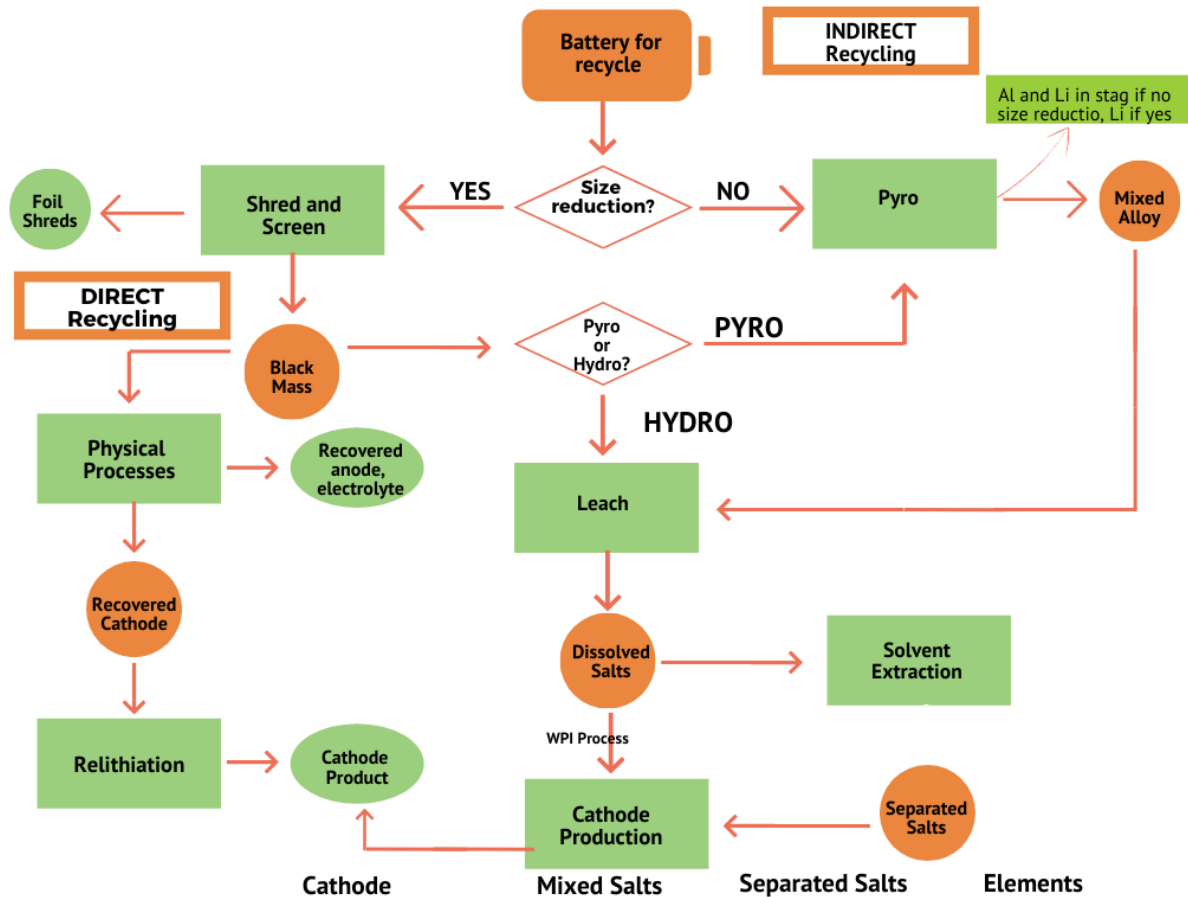
Figure 98 Possible recycling paths for lithium-ion batteries 451
