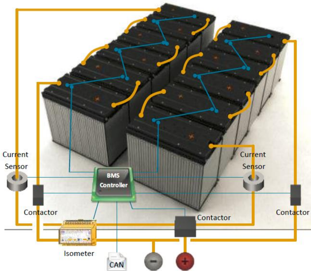
Figure 82: Conceptual illustration of a battery system 370
