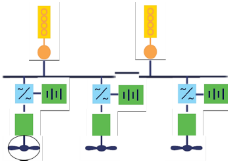
Figure 78: Battery hybrid propulsion with distributed batteries
