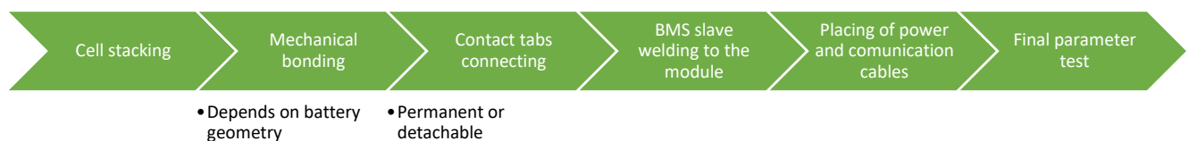
Figure 38 Battery module assembly process
