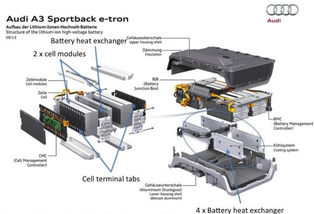
Figure 57 Example of EV Battery 288
