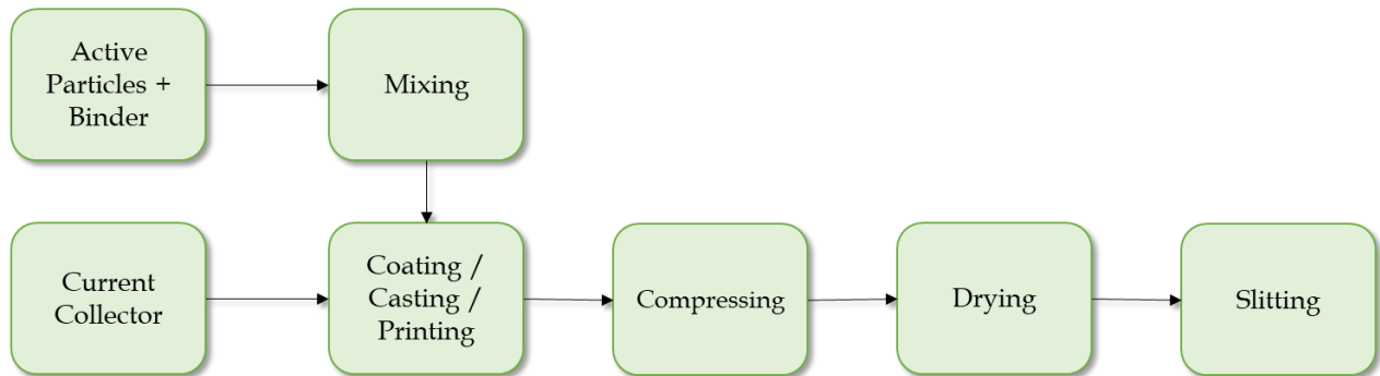
Figure 45 Electrode manufacturing 263 . Flowchart adapted from the source.
