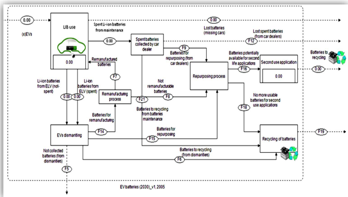
Figure 86: Value chain of EV batteries
