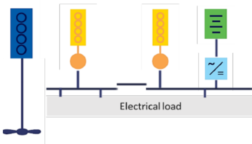
Figure 76: Mechanical propulsion with battery hybrid electric power plant
