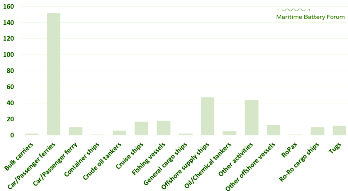
Figure 74: Number of ships with batteries by ship type 367
